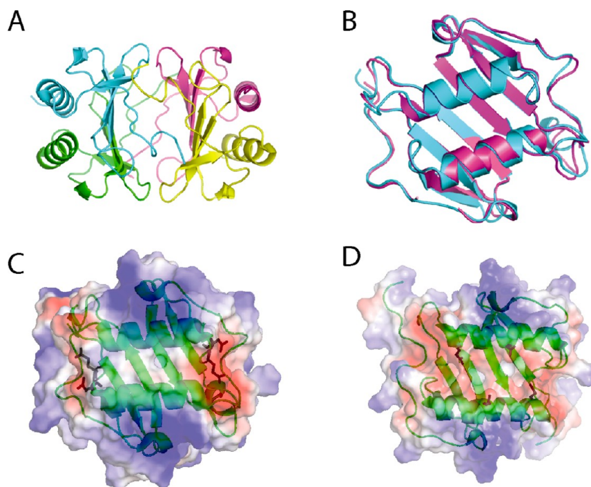
Figure 1. Tertiary structure of MIP-2. A, Four molecules present in the asymmetric unit are represented as ribbons and colored uniquely. Monomers in blue and cyan form one dimer, and the pink and yellow monomers form the other dimer. B, Ribbon structures of superposition of C \alpha atoms of two dimers in the asymmetric unit of the MIP-2 X-ray structure (rmsd 0.54 Å). The superposition was based on matching the secondary structures and calculating an rmsd of the entire structure. C, The electrostatic potential surface of MIP-2. The electronegative region is shaded red and the blue color represents electropositive region. Side chains for D53 and E55 are shown with stick figures for each subunit. D, The electrostatic potential of CXCL8. Side chains for E63 and E70 are shown with stick figures in each subunit. MIP-2 in C is neutral between the helices with increased negative potential in the same location for CXCL8. The side chains for panels C and D are the source of the electronegative potential for MIP-2 and CXCL8, respectively.
