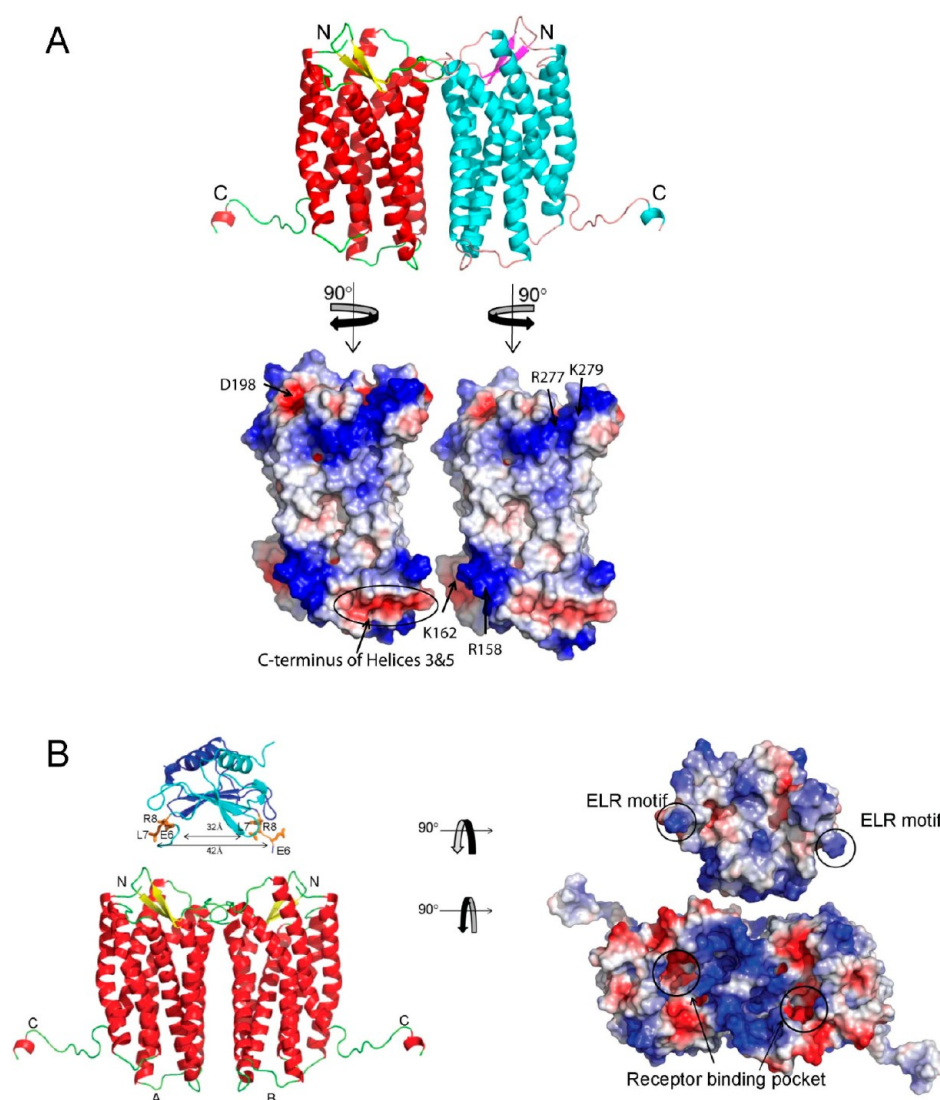
Figure 2. Model of murine CXCR2 dimer bound to MIP-2 dimer. A, Murine CXCR2 was modeled using SWISS-MODEL server with CXCR4 as template (PDB code: 3ODU) and is colored based on secondary structure. The electrostatic potential of the dimer interface is shown in the lower panel. Each monomer surface potential complements the other subunit. B, The orientation of the MIP-2 crystal structure above CXCR2 (A and B represent monomers) is derived from knowledge of the binding sites of each protein. The distance between the binding site cavity for each subunit of CXCR2 receptor overlaps with the distance between each ELR in the MIP-2 dimer. Monomers of MIP2 are represented as ribbon structures (dark blue and cyan), with the side chains of ELR motif as sticks (orange). The CXCR2 and MIP-2 were rotated 90° in opposite direction, and the electrostatic potential was calculated to reveal the potential interacting surfaces (right panel). ELR motifs in the MIP-2 dimers are circled and the arrows in the CXCR2 model represent the potential binding cavity.
