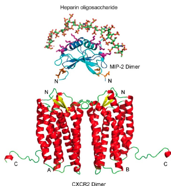
Figure 4. GAG/MIP-2/CXCR2 interface model. The interface of heparin oligosaccharide, MIP-2 chemokine, and CXCR2 is shown in the model. The octadecameric heparin oligosaccharide encompasses the MIP-2 dimer over the helices. The monomers of MIP-2 are represented as ribbons (dark blue and light blue) with the side chains of heparin-interacting residues and the ELR motif as sticks (pink and orange, respectively). The heparin oligosaccharide MIP-2 model was aligned to MIP-2 of the MIP-2/CXCR2 complex (Figure 2) to obtain the tertiary model complex. The heparin oligosaccharide/MIP-2 interaction stabilizes MIP-2 dimer and does not interfere with binding to CXCR2.
