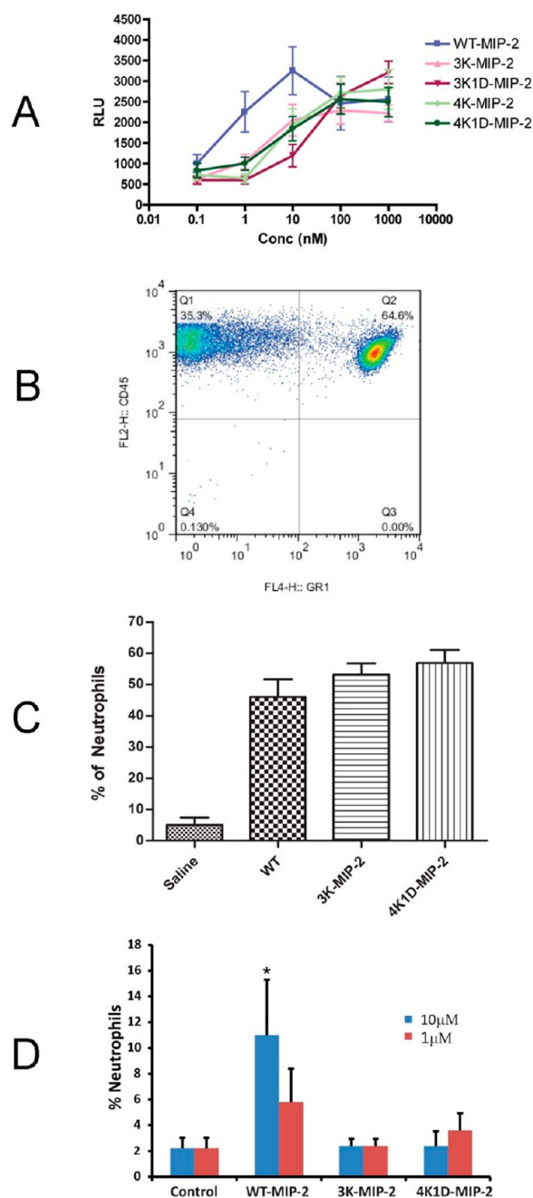
Figure 5. In vitro and in vivo chemotaxis effects of MIP-2 GAG-deficient mutants. A, In vitro chemotaxis of neutrophils in response to WT and MIP-2 mutants at various concentrations. The migrated neutrophils were measured by luminescence represented as relative luminescence unit (RLU). The graph represents the mean of three different experiments done in triplicate (***, p < 0.0001 ; *, p < 0.01 ). B, C and D, Effects of GAG-deficient mutations of MIP-2 in vivo. B, Representative FACS analysis of neutrophils (CD45 + GR1 + ) recruited to the peritoneum in response to 300 ng IP injection of WT. C, Percentage of neutrophils recruited to the peritoneum in response to WT, 3K-MIP-2, and 4K1D-MIP-2. D, Percentage of neutrophils recruited in BAL in response to instillation of 1 \mu M or 10 \mu M of WT MIP-2 or GAG-deficient mutants 3K-MIP-2, and 4K1D-MIP-2. The in vivo data represent the mean number of neutrophils from six female BALB/c mice of 8–10 weeks of age.
