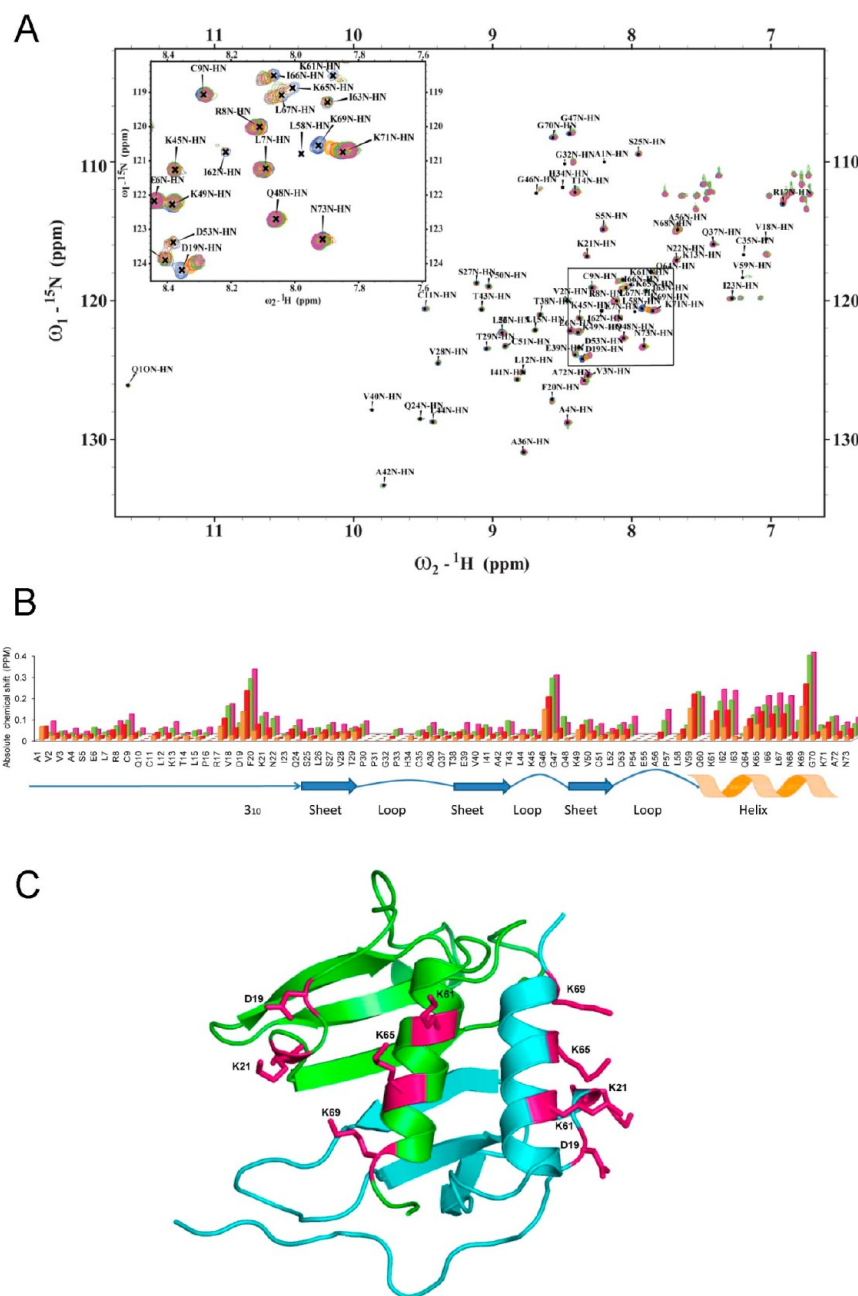
Figure 3. NMR spectroscopic studies of murine MIP-2 and heparin disaccharide interaction. A, NMR chemical shift changes induced by titration of heparin disaccharide I-S. ^1\text{H} - ^{15}\text{N} -HSQC spectra of 300\ \mu\text{M} ^{15}\text{N} -MIP-2 (blue) are overlaid with spectra from molar ratios of ^{15}\text{N} -MIP-2 to disaccharide of 1:2, 1:4, 1:8, and 1:16 (orange, red, green, and pink), respectively. Peak labels indicate peaks for the uncomplexed (apo) protein. B, Absolute NMR chemical shift change of each residue for the disaccharide titration. Absolute NMR chemical shift change for each ratio are calculated as ((\text{I}|\text{Nppm-bound} - \text{Nppm-apo}) + (\text{Hppm-bound} - \text{Hppm-apo} \times 6.5))/2 . Uncomplexed ^{15}\text{N} -MIP-2 compared to ^{15}\text{N} -MIP-2:heparin disaccharide I-S ratios of 1:2 (orange), 1:4 (red), 1:8 (green), and 1:16 (pink). Changes in NMR chemical shifts for proline residues are reported as zero as they lack an amide proton. Regions of secondary structure are indicated below with block arrows representing \beta regions and zigzags representing helical regions. C, The chemical shifts are mapped and the residues are shown as sticks on a ribbon diagram of the crystallographic dimeric (green and blue monomers) structure of MIP-2.
